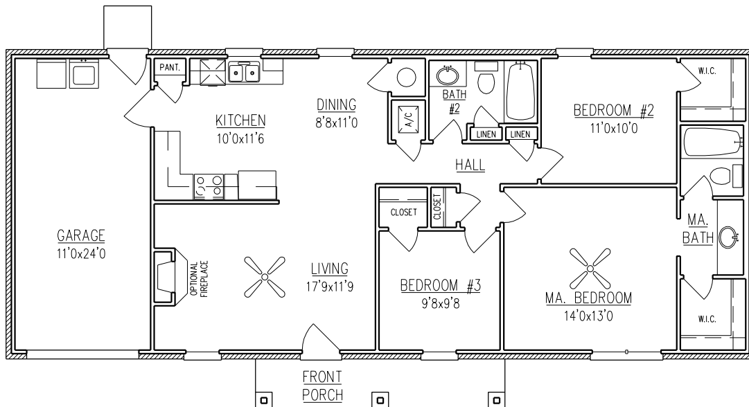
FLOOR PLAN
