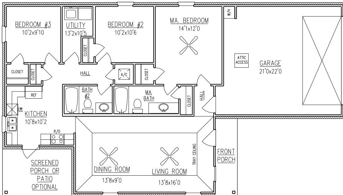
FLOOR PLAN
