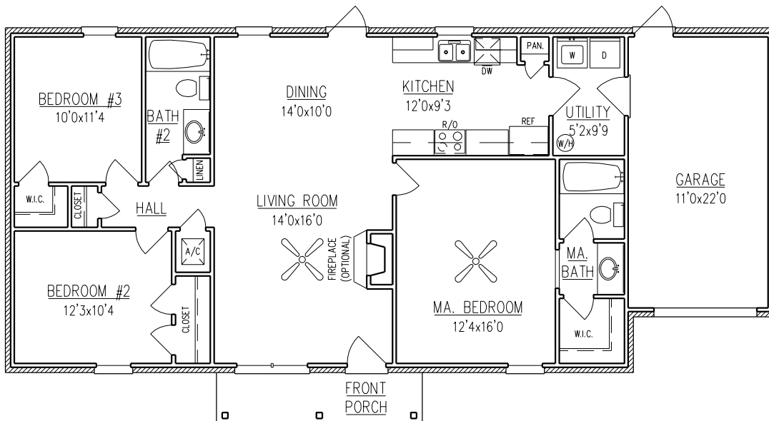
FLOOR PLAN
