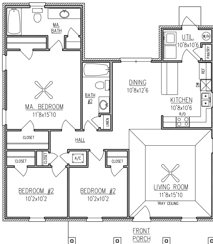
FLOOR PLAN
