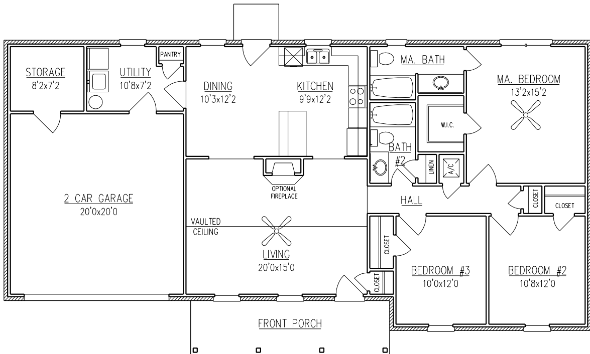
FLOOR PLAN
