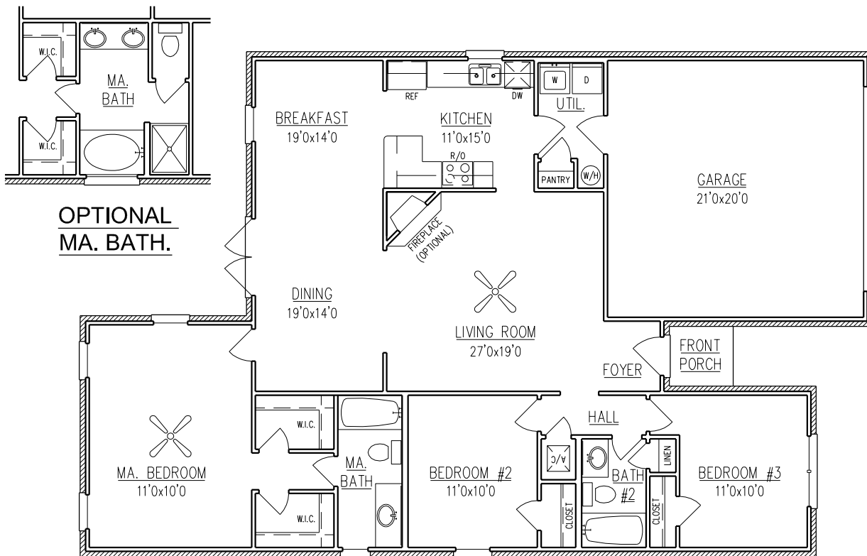
FLOOR PLAN
