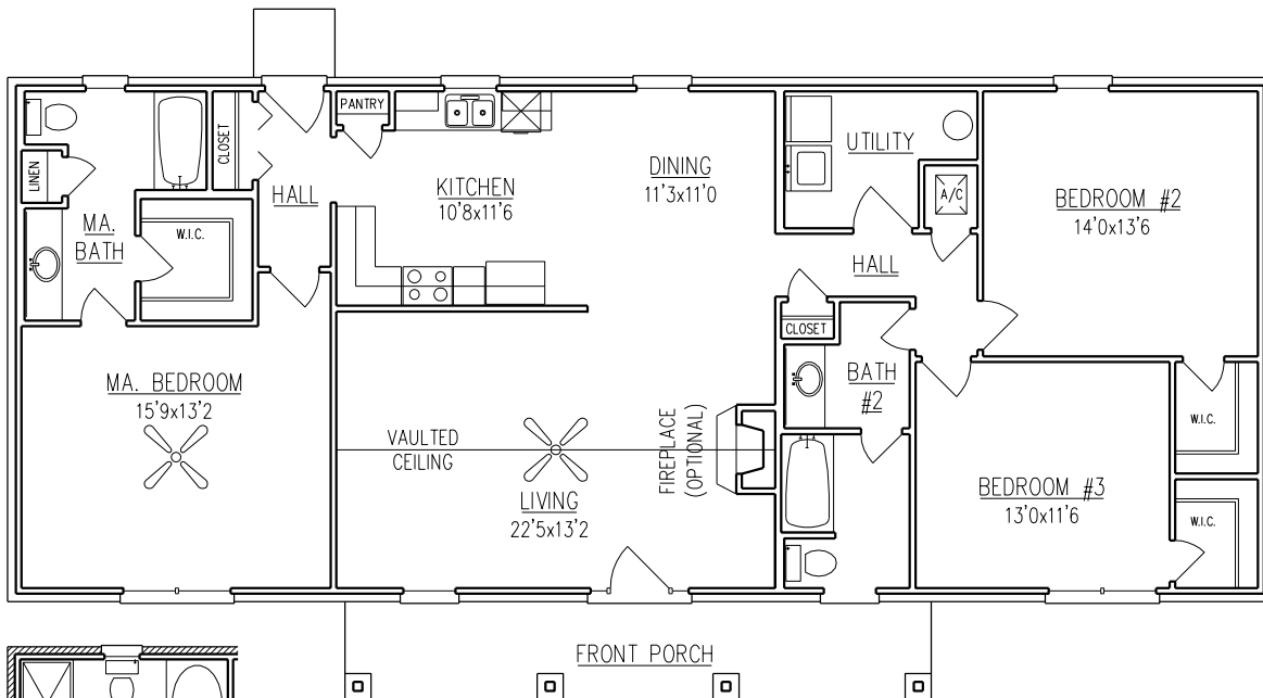
FLOOR PLAN
