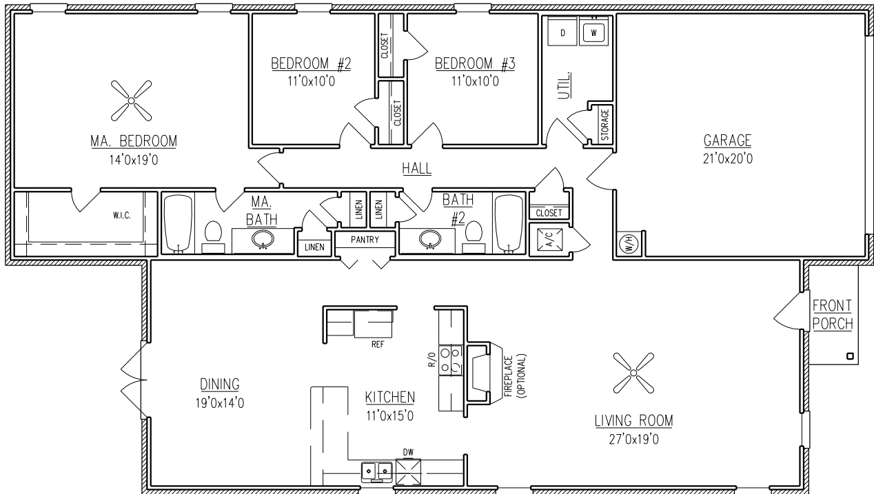
FLOOR PLAN
