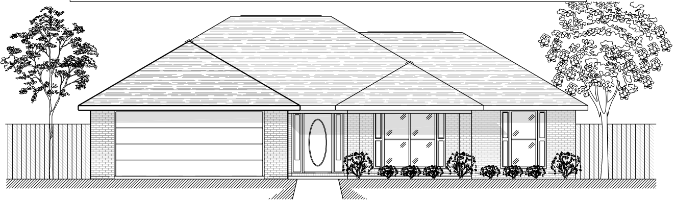
ELEVATION (A)
